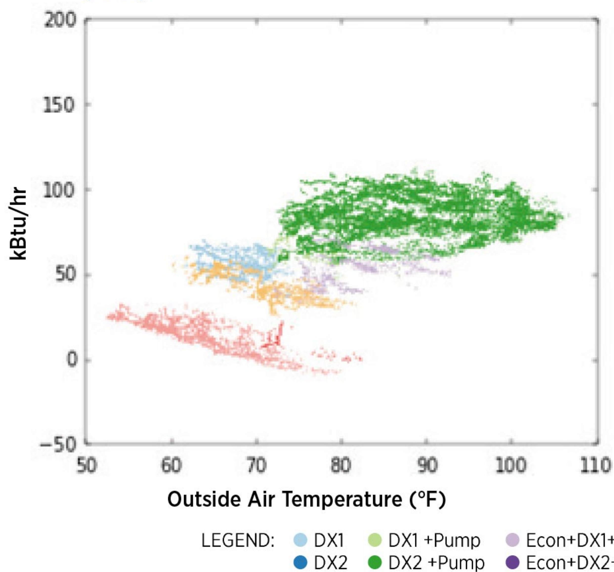
FIGURE 3: SENSIBLE ROOM COOLING CAPACITY (AC7)
