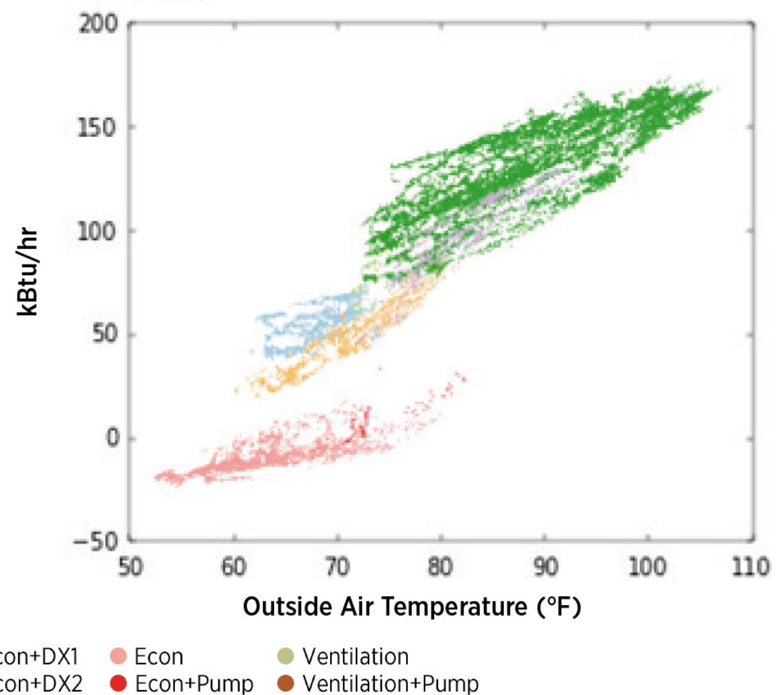
FIGURE 4: SENSIBLE SYSTEM COOLING CAPACITY (AC7)
